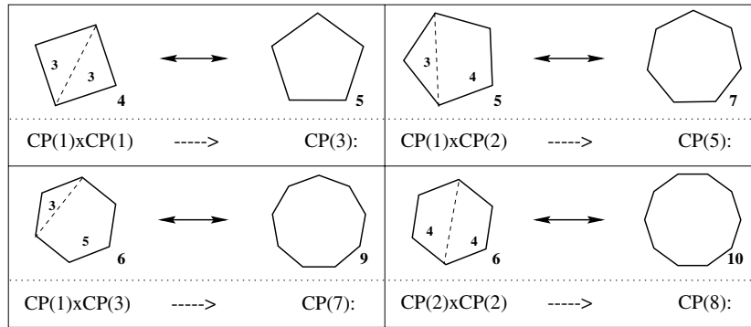
Figure 1. Combination of shapes and their entangled configurations. When a pair of shapes are combined, the resulting shapes of the disentangled states have four points that are collinear, as indicated on the left-hand side. The right-hand side shapes correspond to entangled states. In general, entangled shapes have a larger number of points than the sum of the numbers of points associated with individual disentangled shapes.
